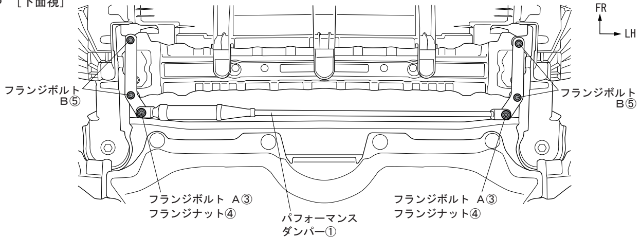
図5 [下面視]
